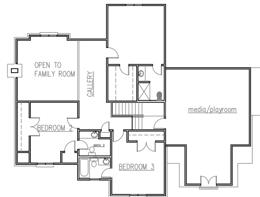
SECOND FLOOR (1785 sf)
