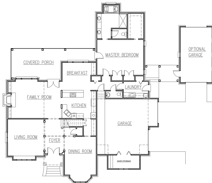
FIRST FLOOR (2233 sf)
