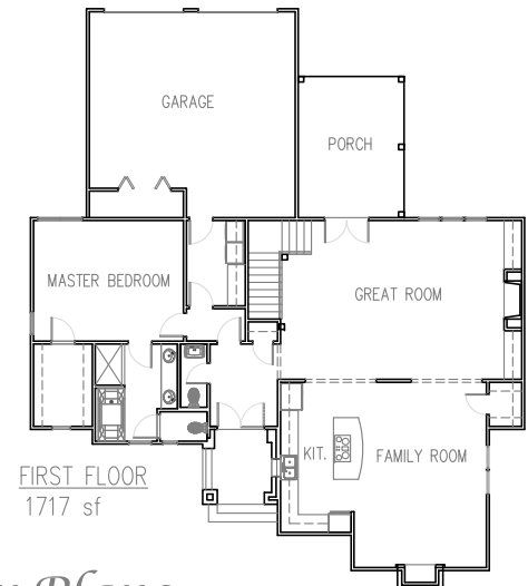
Floor Plans
