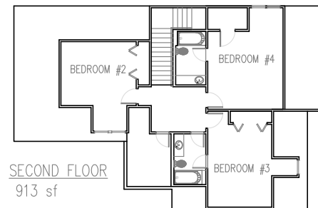
Floor Plans
