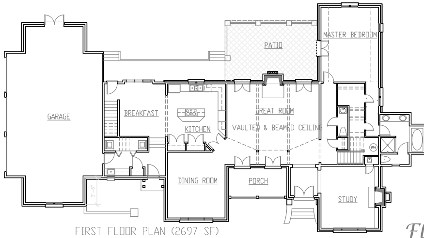
FIRST FLOOR PLAN (2697 SF)
