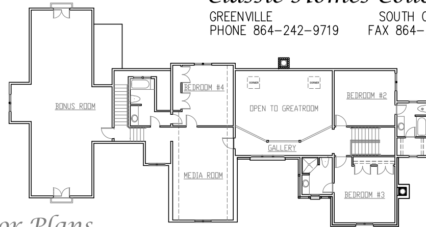
SECOND FLOOR (1633 SF)
