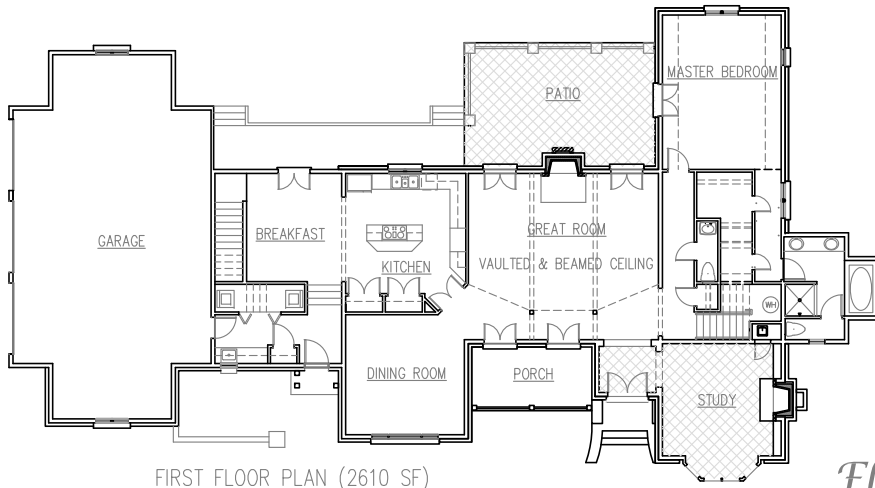
FIRST FLOOR PLAN (2610 SF)
