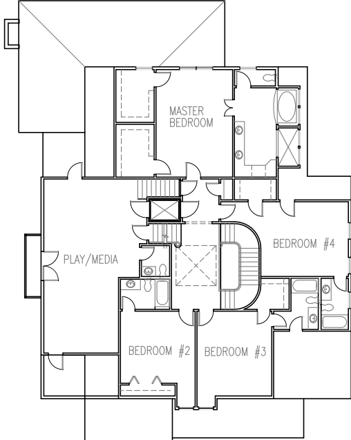
Second Floor Plan (2395 s.f. heated )
