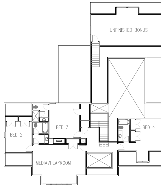
SECOND FLOOR 1544 S.F.
