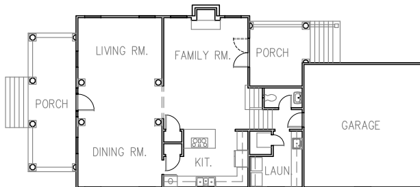
First Floor Plan 1227 SF
